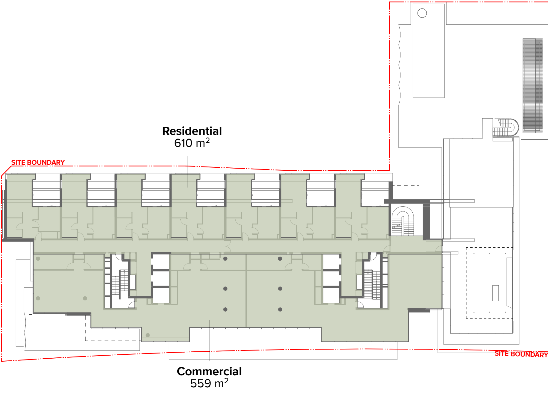
Level 03 GFA : 1169m²
