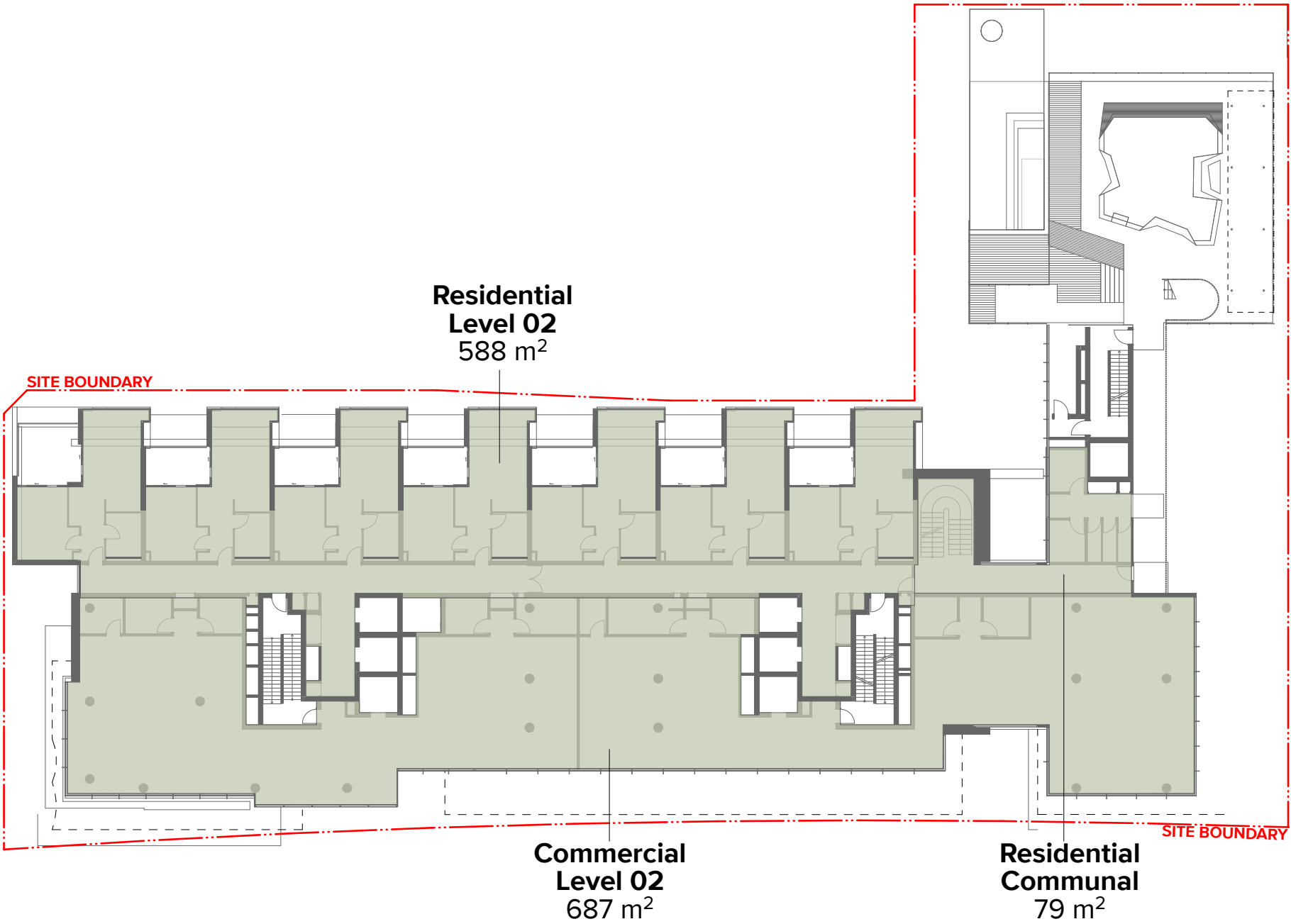
Level 02 GFA : 1354m²
